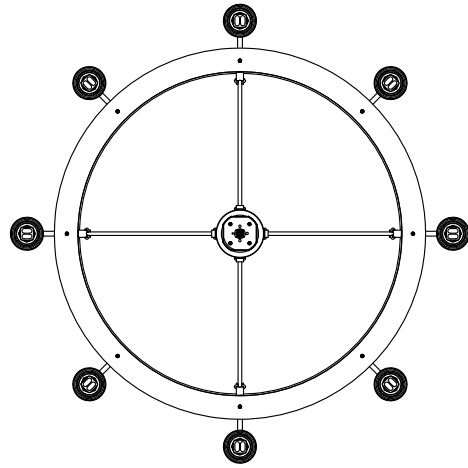
LAMPING LAYOUT - FLUORESCENT
