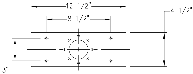
MOUNTING DETAIL
